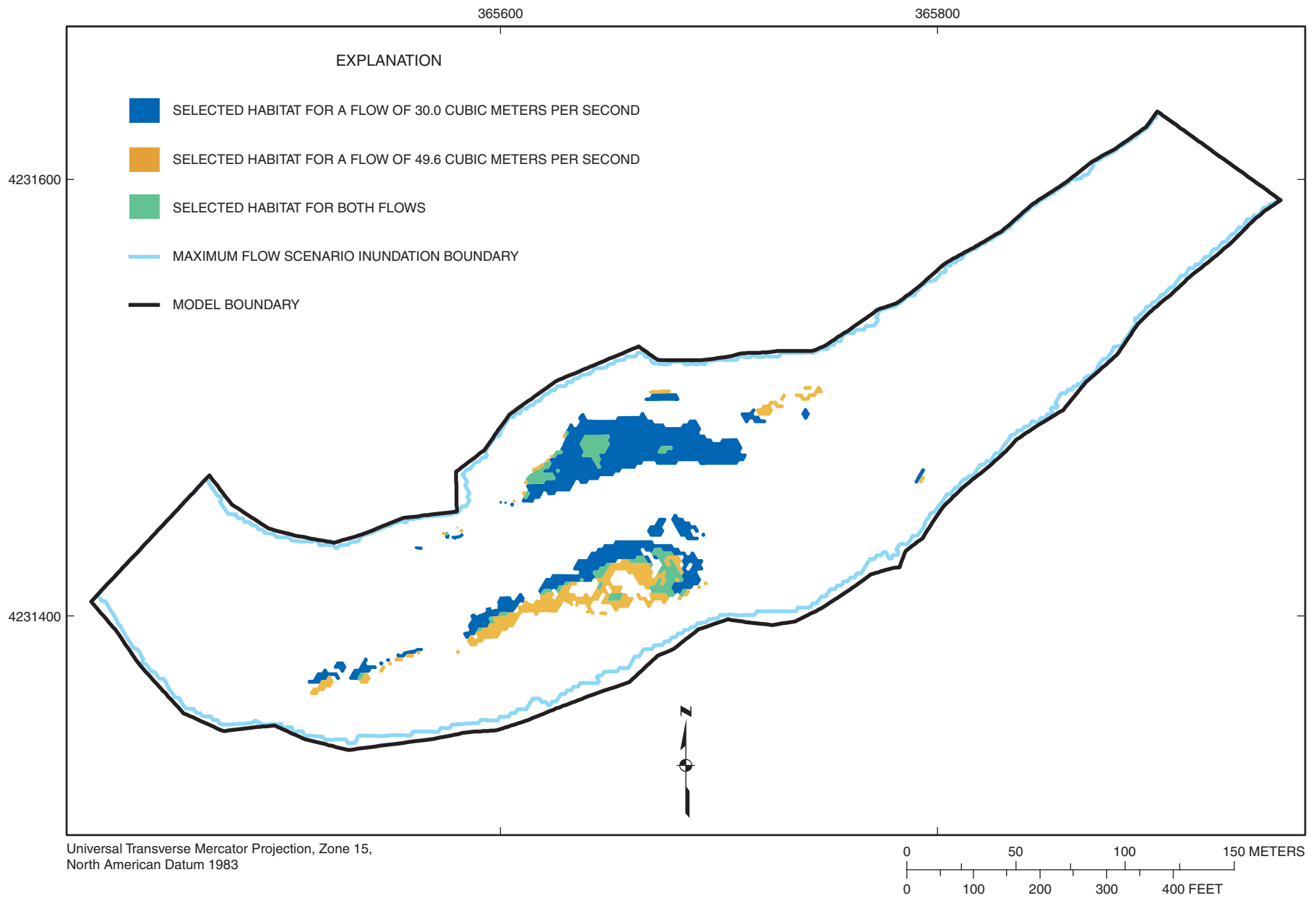
Figure 4-8. Selected habitat area distribution for habitat category 1 (suckermouth minnow) at flows of 30.0 and 49.6 cubic meters per second at Marais des Cygnes River site MDC2.
